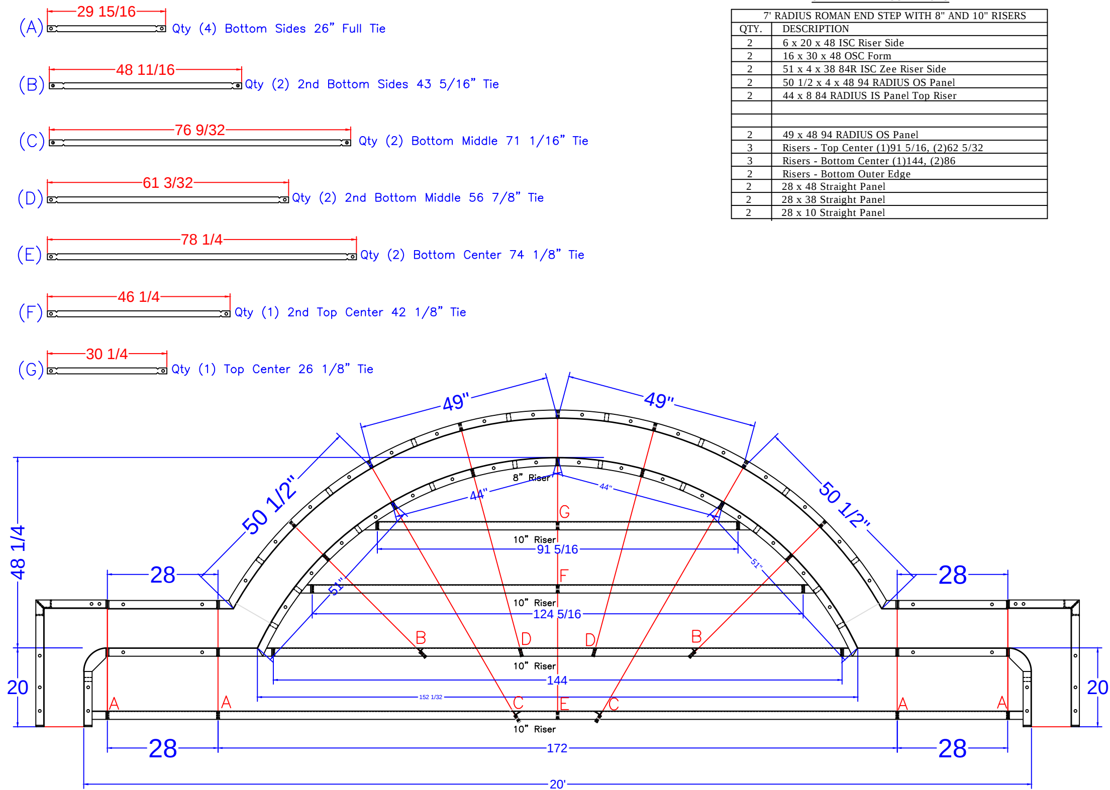
7' RADIUS ROMAN END STEP DETAIL SCALE: 1' = 1/2"
