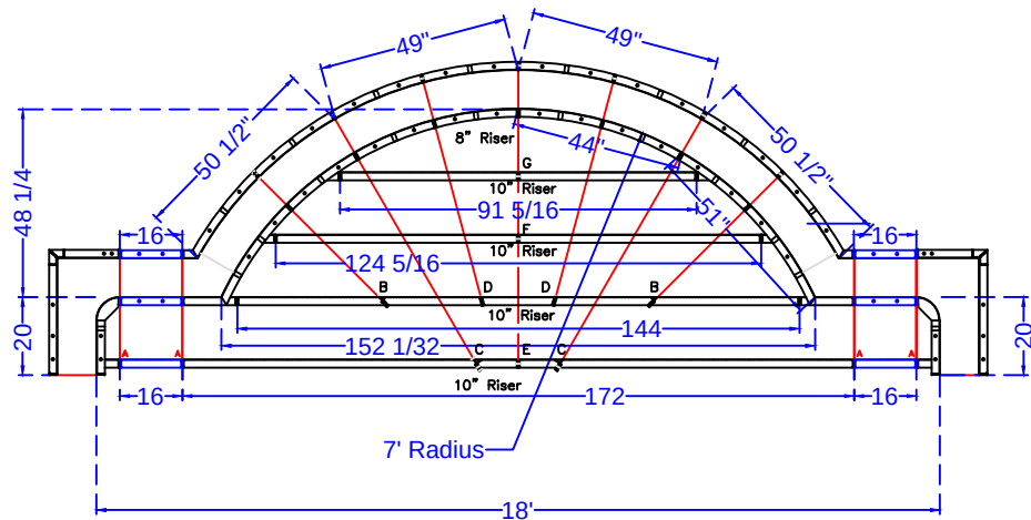
18' ROMAN END STEP ASSEMBLY SHOWN x 48 SCALE: 1' = 1/4"
