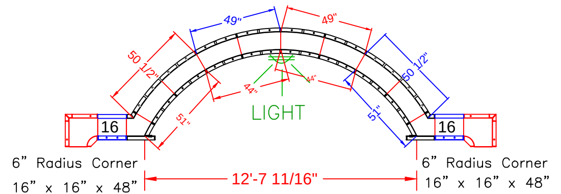
18' ROMAN END ASSEMBLY SHOWN x 48 SCALE: 1' = 1/4"
