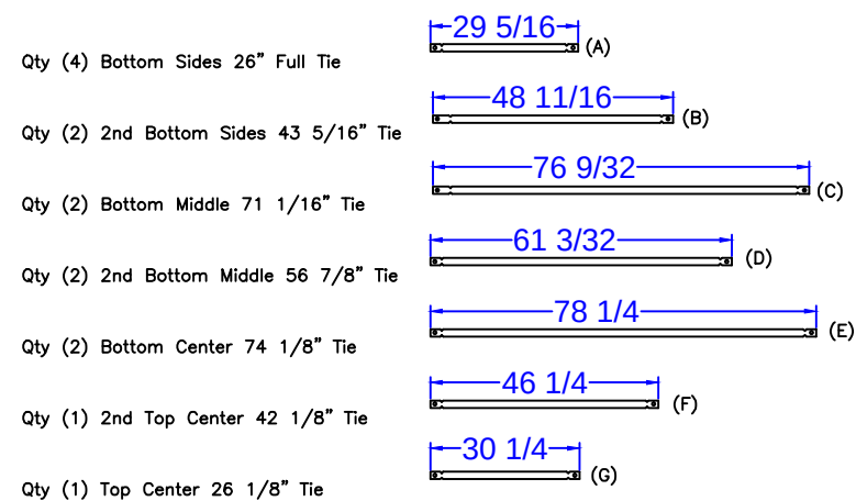
18' ROMAN END STEP - TIES SCALE: 1' = 1/4"
