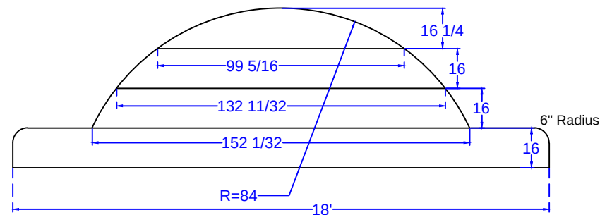
STEP DETAIL SCALE: 1' = 1/4"
