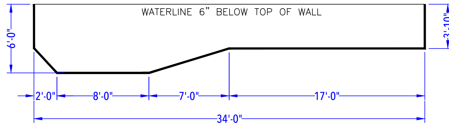
DEPTH DETAIL
