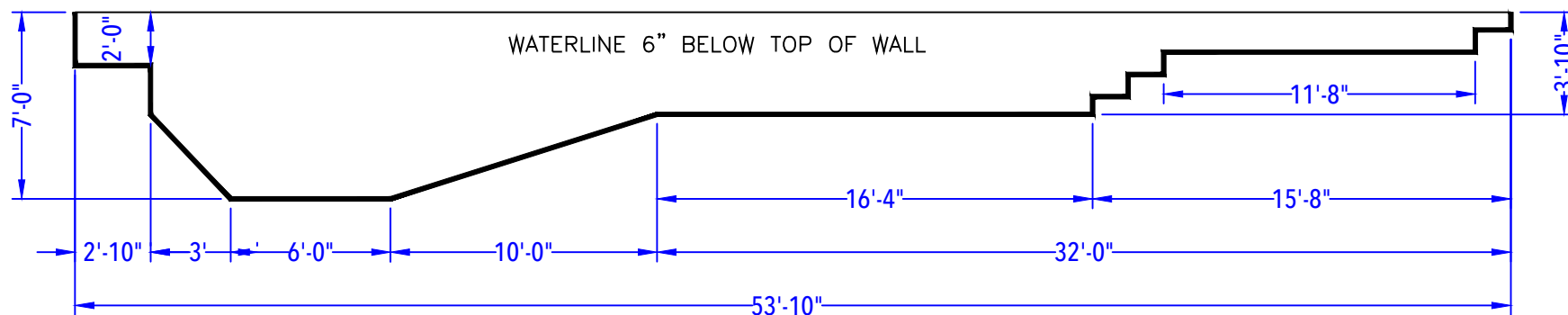
DEPTH DETAIL
