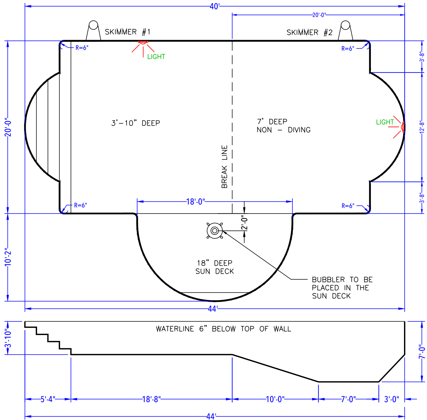
DEPTH DETAIL
