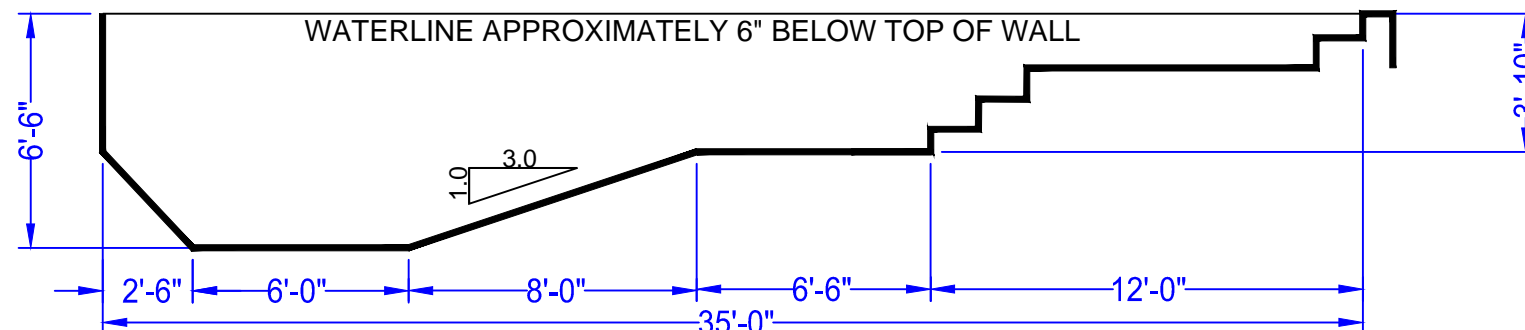
DEPTH DETAIL
