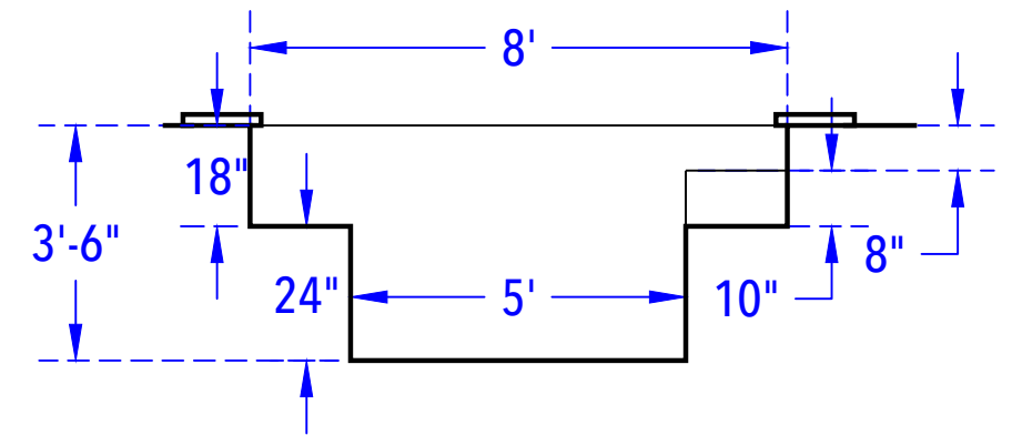
SPA ELEVATION (After Bottom & Plaster) N.T.S
