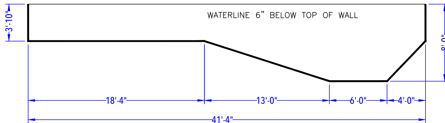
DEPTH DETAIL
