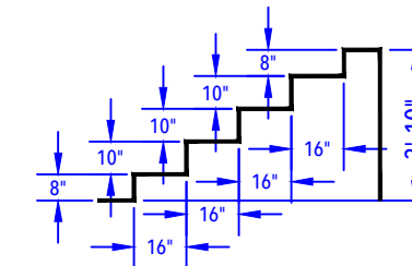
ENTRY STEP DETAIL (After Concrete & Liner) N.T.S.
