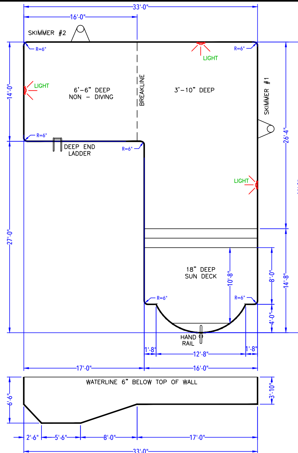
DEPTH DETAIL
