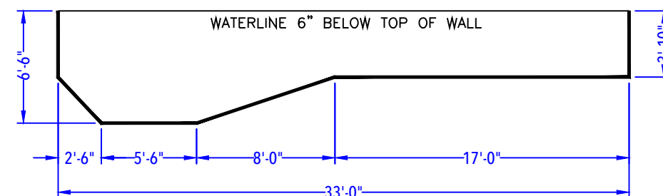
DEPTH DETAIL
