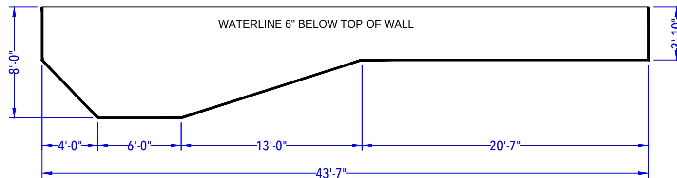
DEPTH DETAIL
