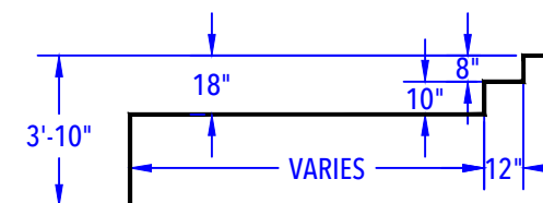
SIDE SUN DECK DETAIL (After Concrete & Liner) N.T.S.
