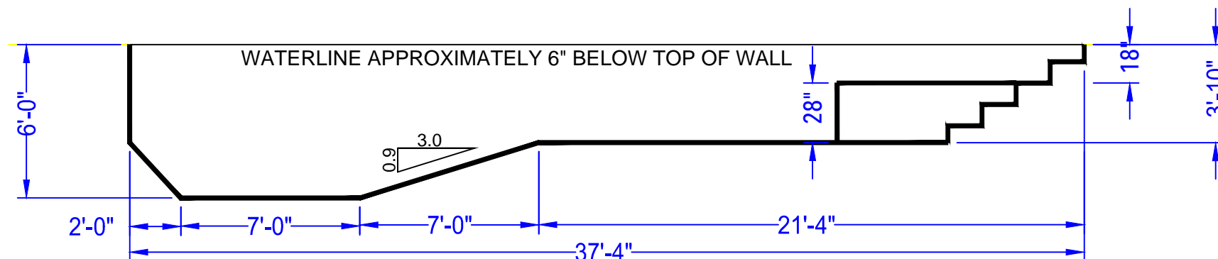
DEPTH DETAIL
