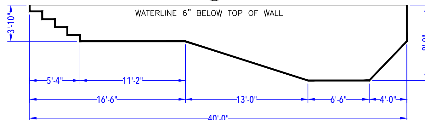
DEPTH DETAIL
