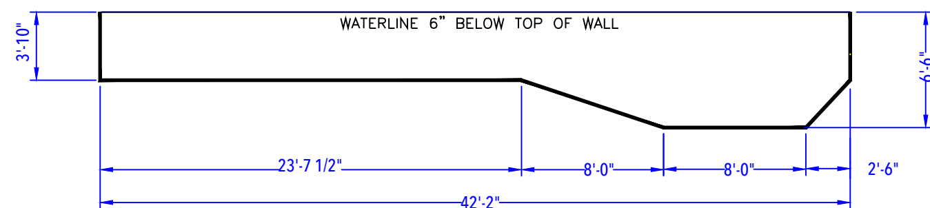
DEPTH DETAIL
