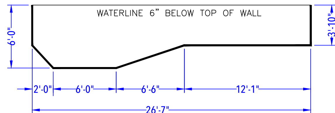
DEPTH DETAIL
