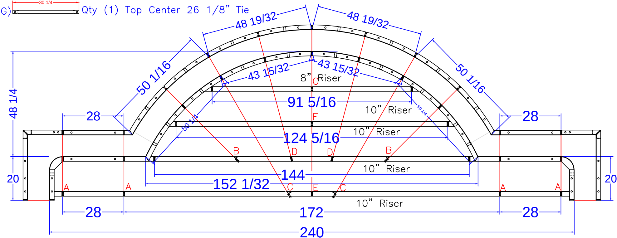
7' RADIUS ROMAN END STEP DETAIL SCALE: 1' = 1/4"
