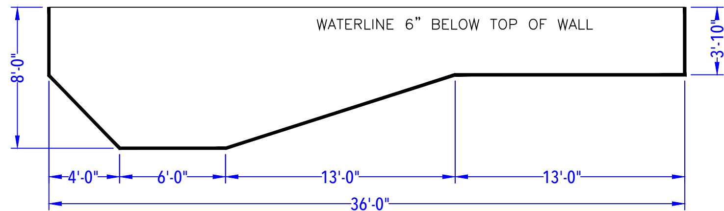
DEPTH DETAIL
