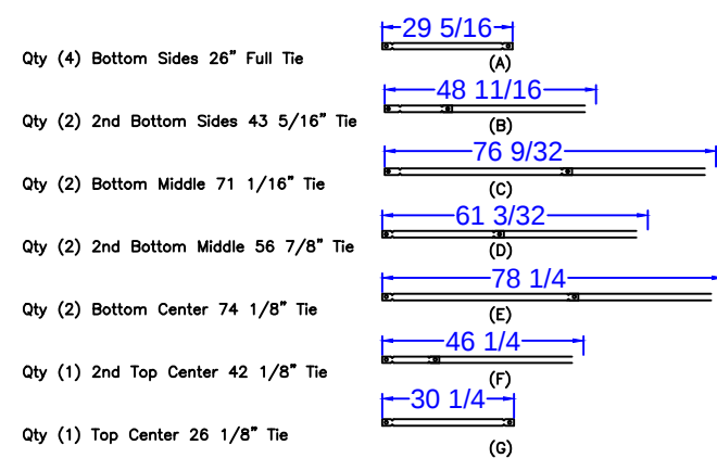
18' ROMAN END STEP - TIES
