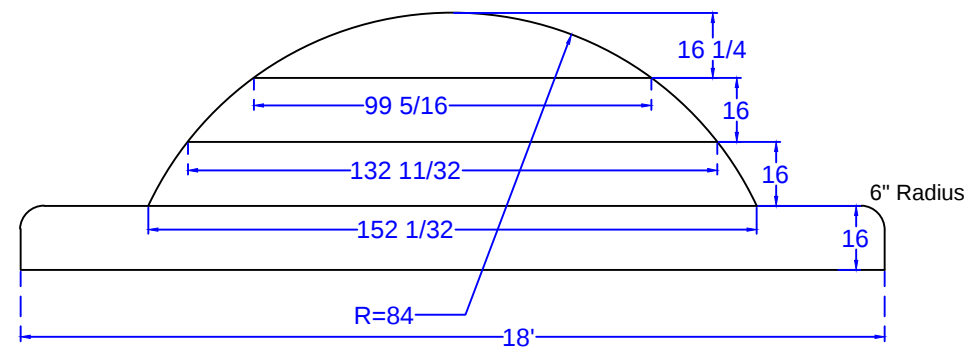
STEP DETAIL
