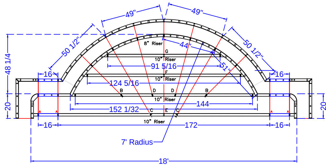
18' ROMAN END STEP ASSEMBLY SHOWN x 48
