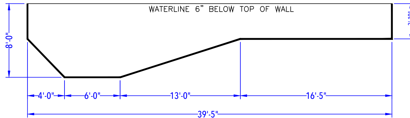
DEPTH DETAIL
