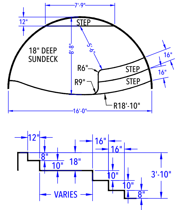
SUN DECK & ENTRY STEP DETAIL (After Concrete & Liner) N.T.S.
