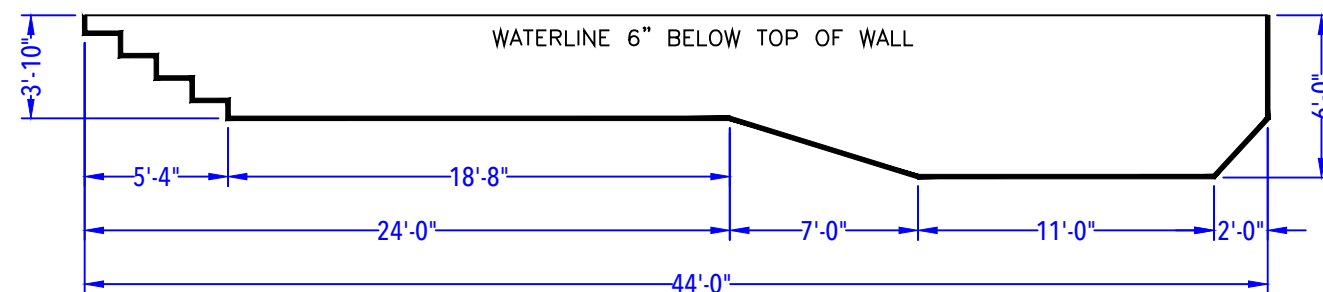
DEPTH DETAIL
