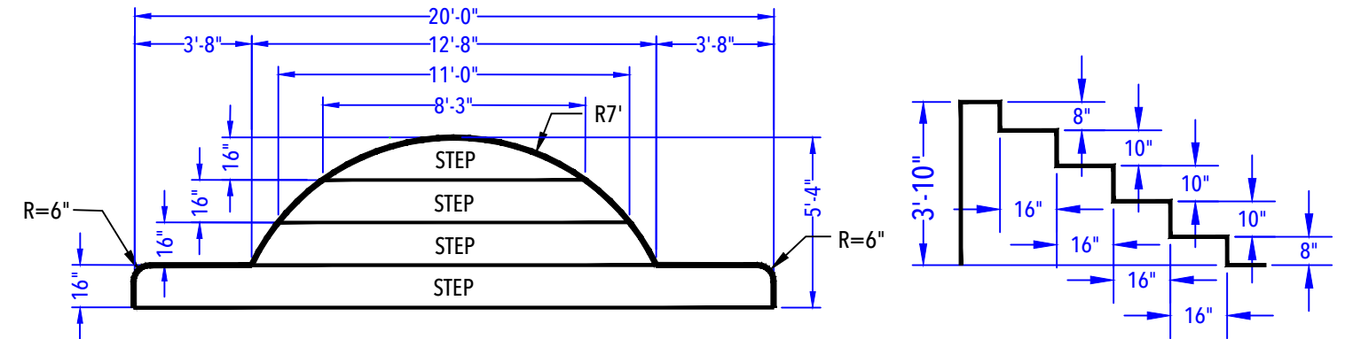
ENTRY STEP DETAIL (After Concrete & Liner) N.T.S.
