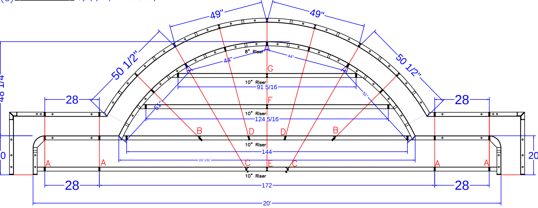
7' RADIUS ROMAN END STEP DETAIL
