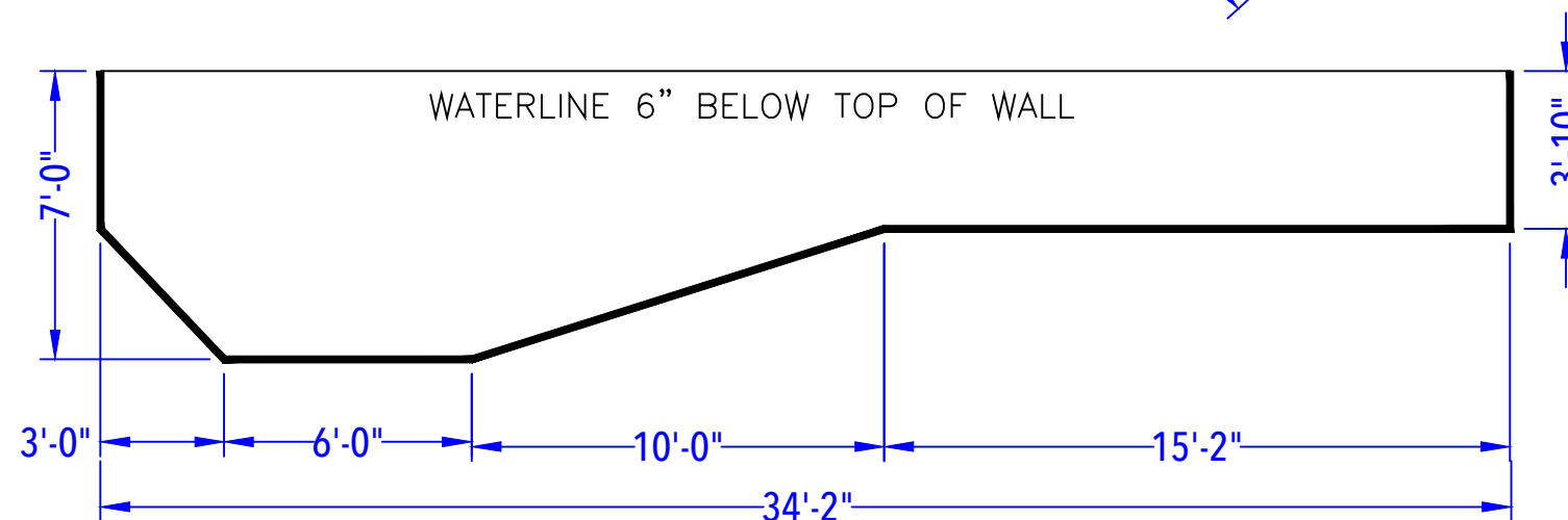
DEPTH DETAIL
