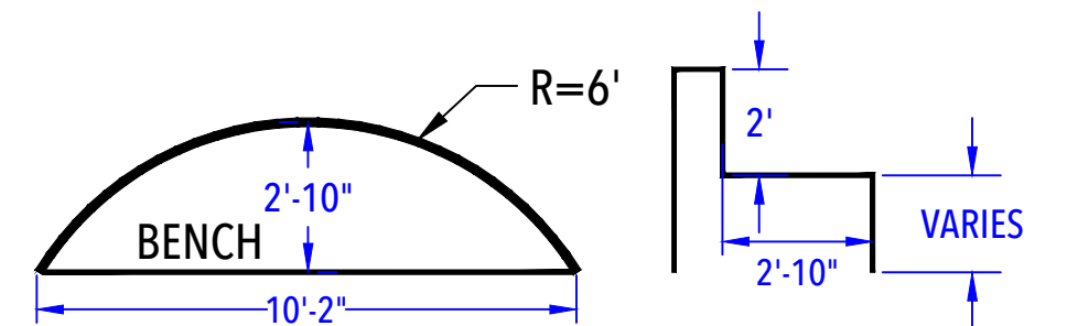
ENTRY STEP DETAIL (After Concrete & Liner) N.T.S.
