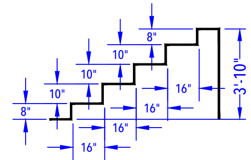
STEP DETAIL (After Bottom & Liner) N.T.S.
