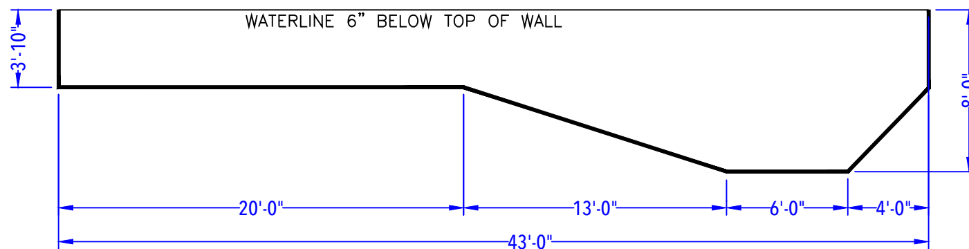
DEPTH DETAIL
