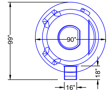
SPA DETAIL (After Concrete & Liner) N.T.S.
