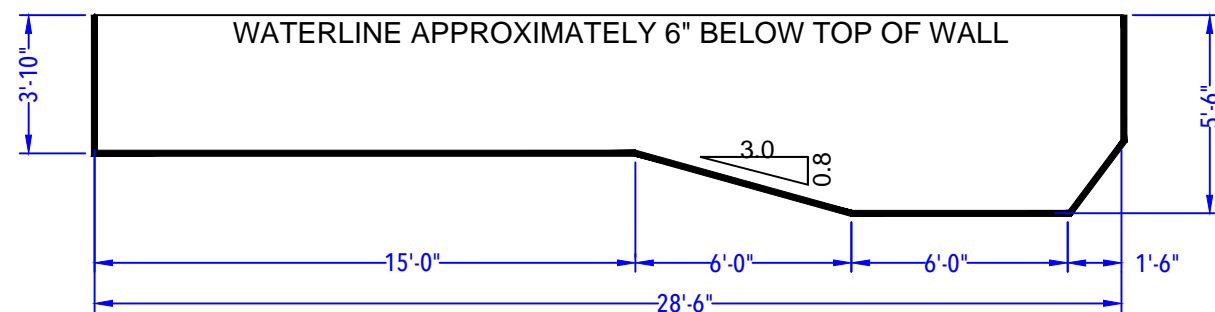
DEPTH DETAIL
