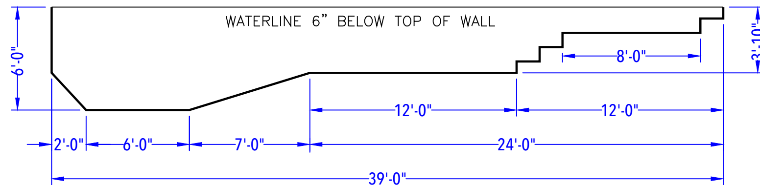
DEPTH DETAIL
