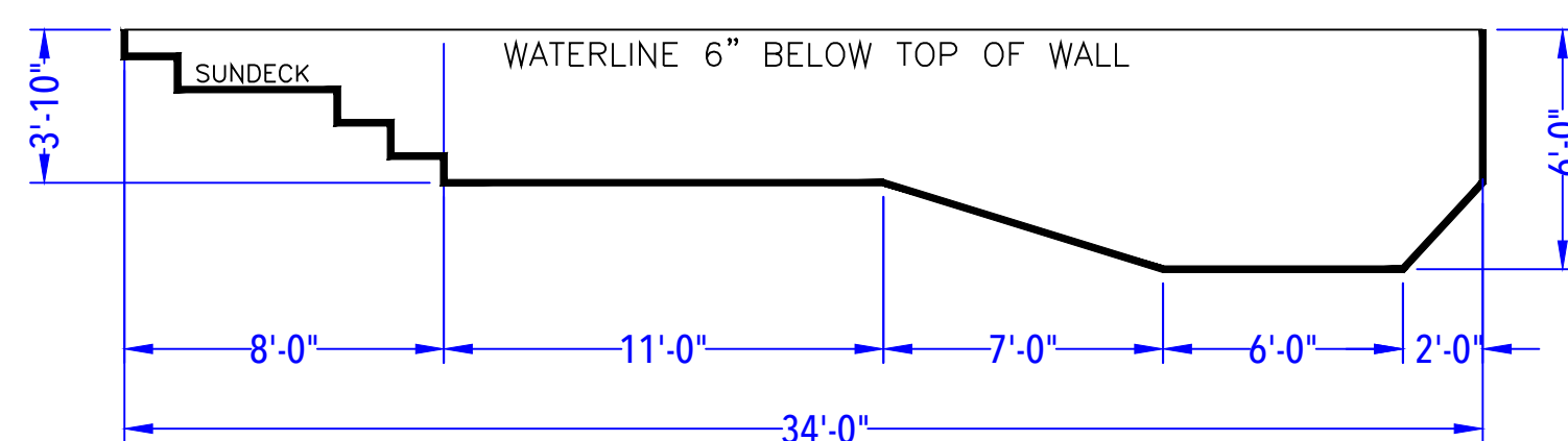
DEPTH DETAIL
