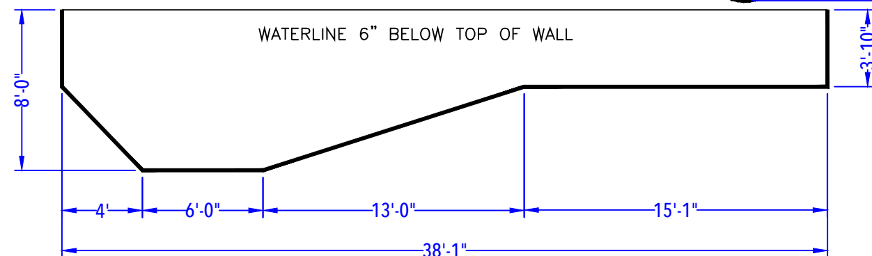
DEPTH DETAIL
