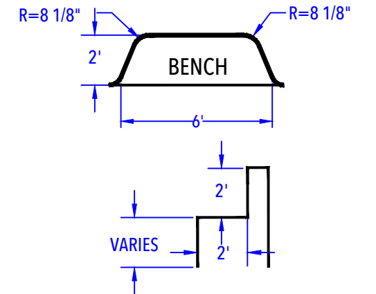
SHALLOW END BENCH DETAIL (After Concrete & Liner) N.T.S.
