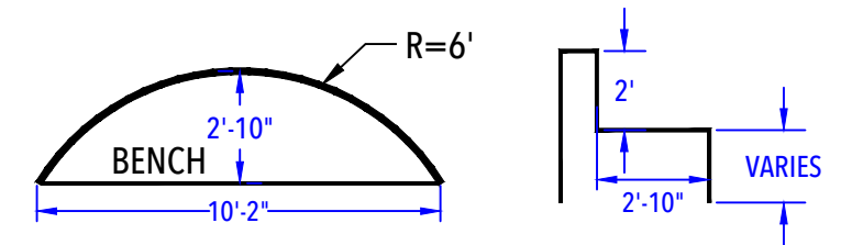
DEEP END BENCH DETAIL (After Concrete & Liner) N.T.S.
