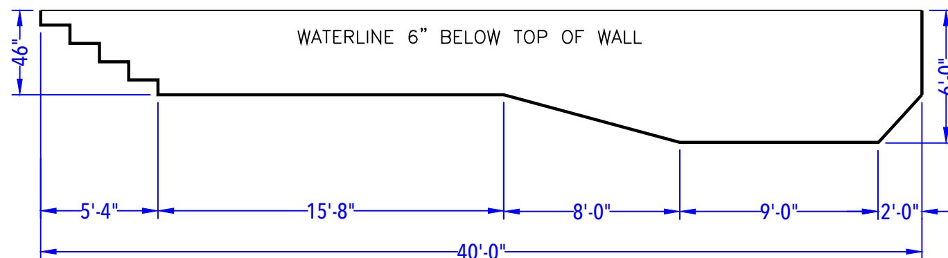
DEPTH DETAIL
