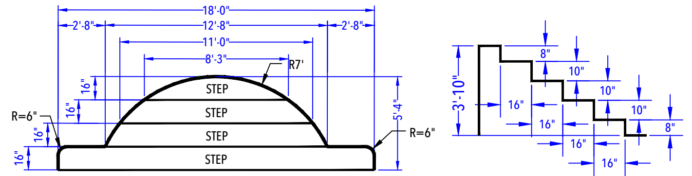
ENTRY STEP DETAIL (After Concrete & Liner) N.T.S.
