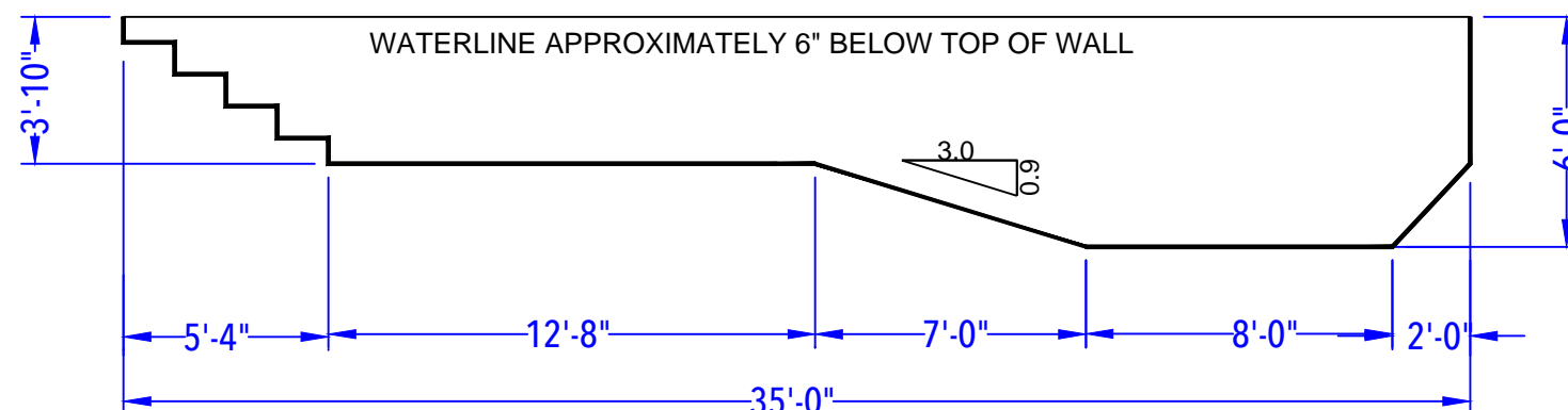
DEPTH DETAIL
