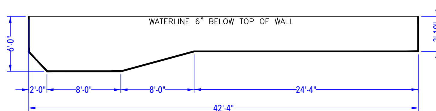
DEPTH DETAIL
