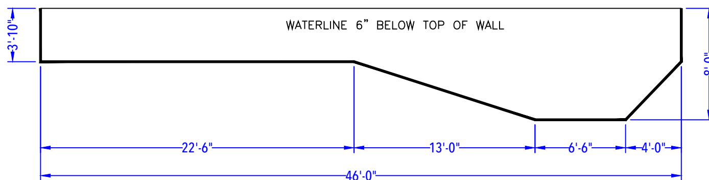
DEPTH DETAIL
