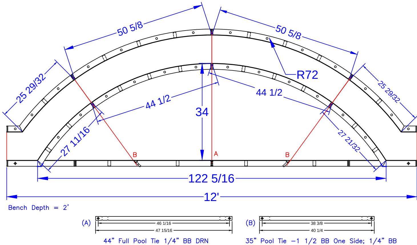
10'-2" ROMAN END LOVE SEAT (6' RADIUS) SCALE: 1' = 1/2"
