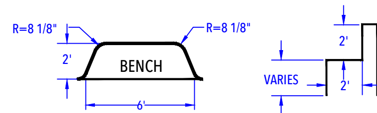
SHALLOW END BENCH DETAIL (After Concrete & Liner) N.T.S.
