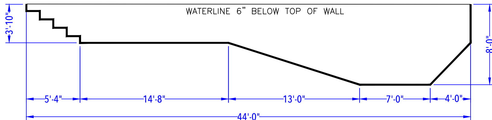
DEPTH DETAIL
