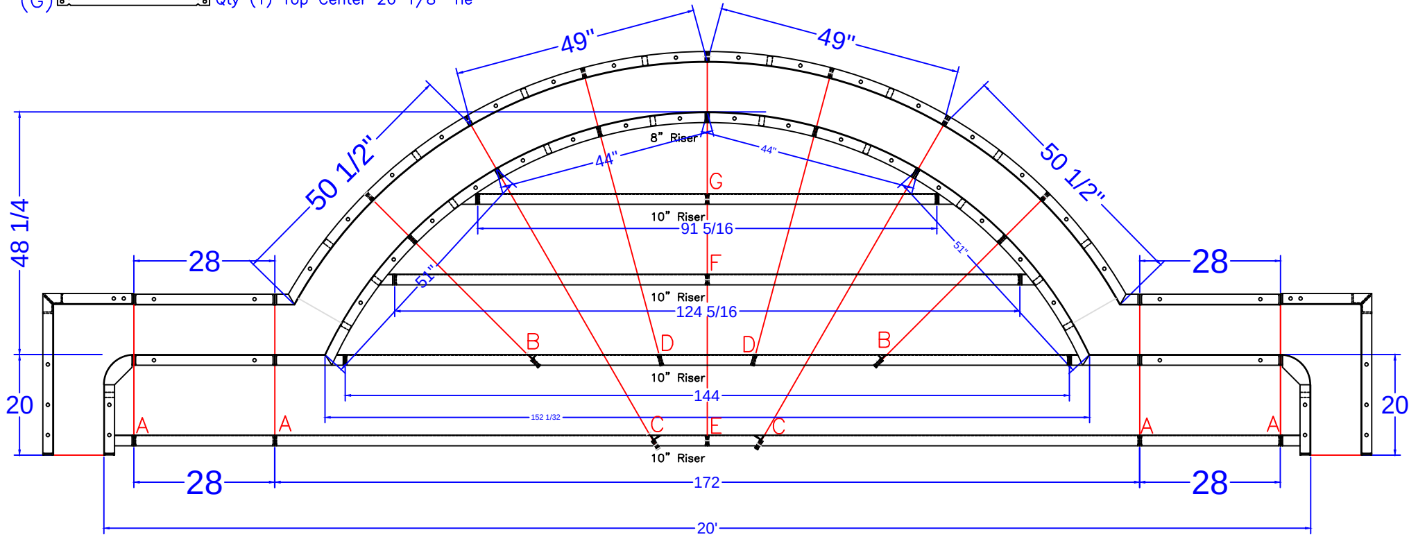
7' RADIUS ROMAN END STEP DETAIL
