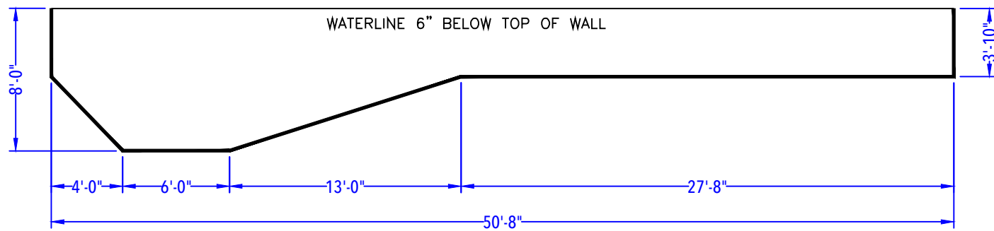
DEPTH DETAIL
