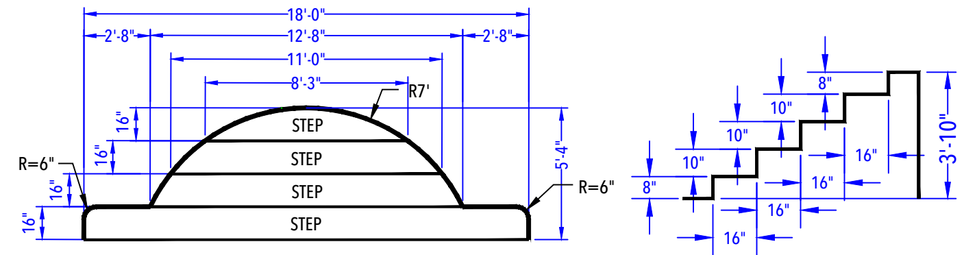
ENTRY STEP DETAIL (After Concrete & Liner) N.T.S.
