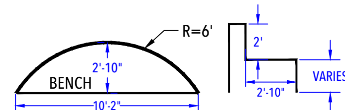
DEEP END BENCH DETAIL (After Concrete & Liner) N.T.S.
