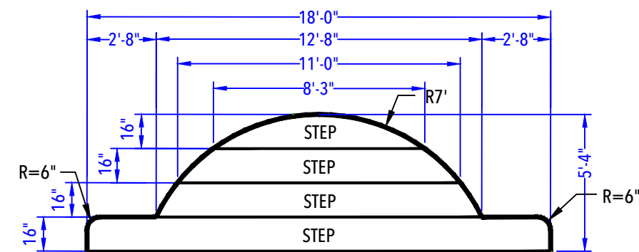
ENTRY STEP DETAIL (After Concrete & Liner) N.T.S.
