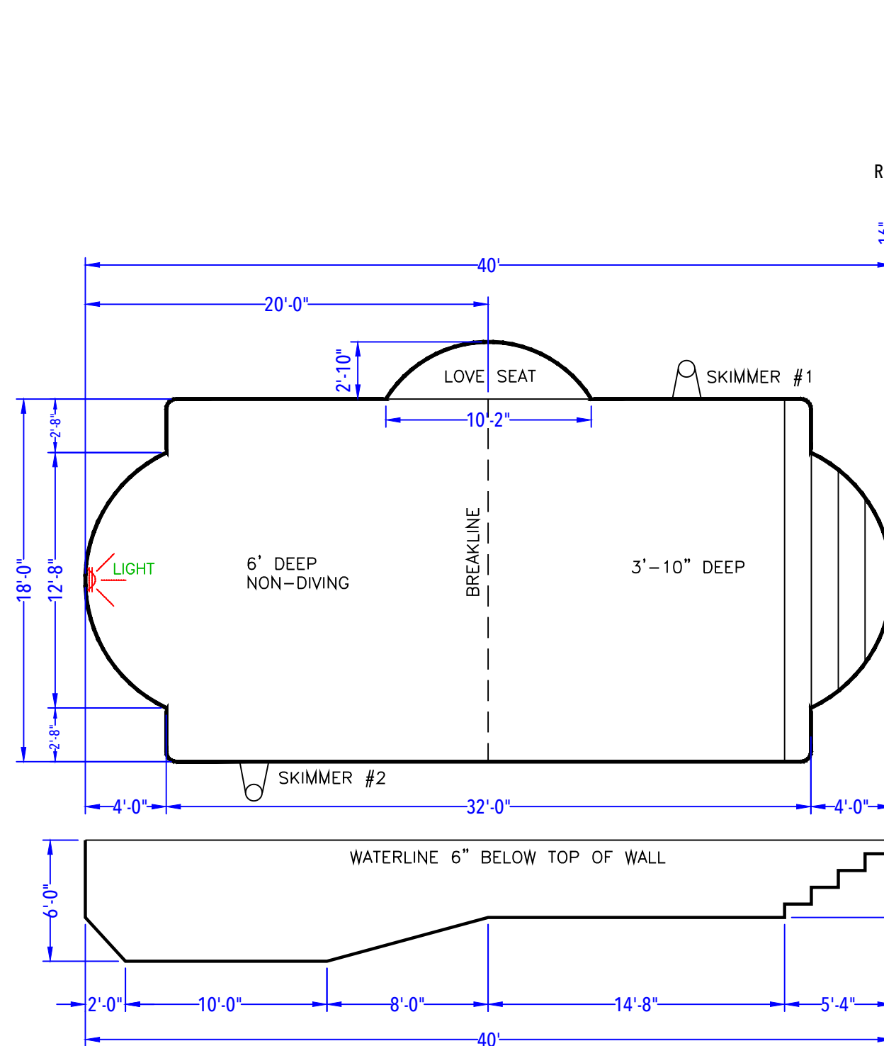
DEPTH DETAIL
