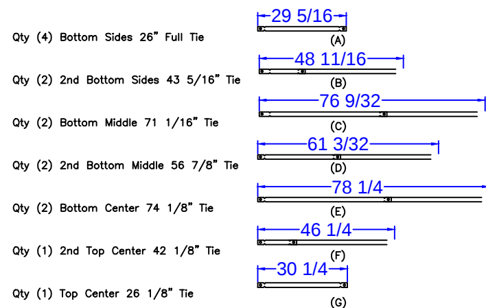
18' ROMAN END STEP - TIES SCALE: 1' = 1/4"
