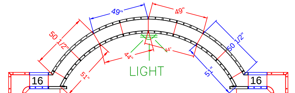
18' ROMAN END ASSEMBLY SHOWN x 48 SCALE: 1' = 1/4"
