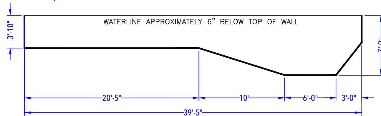
DEPTH DETAIL
