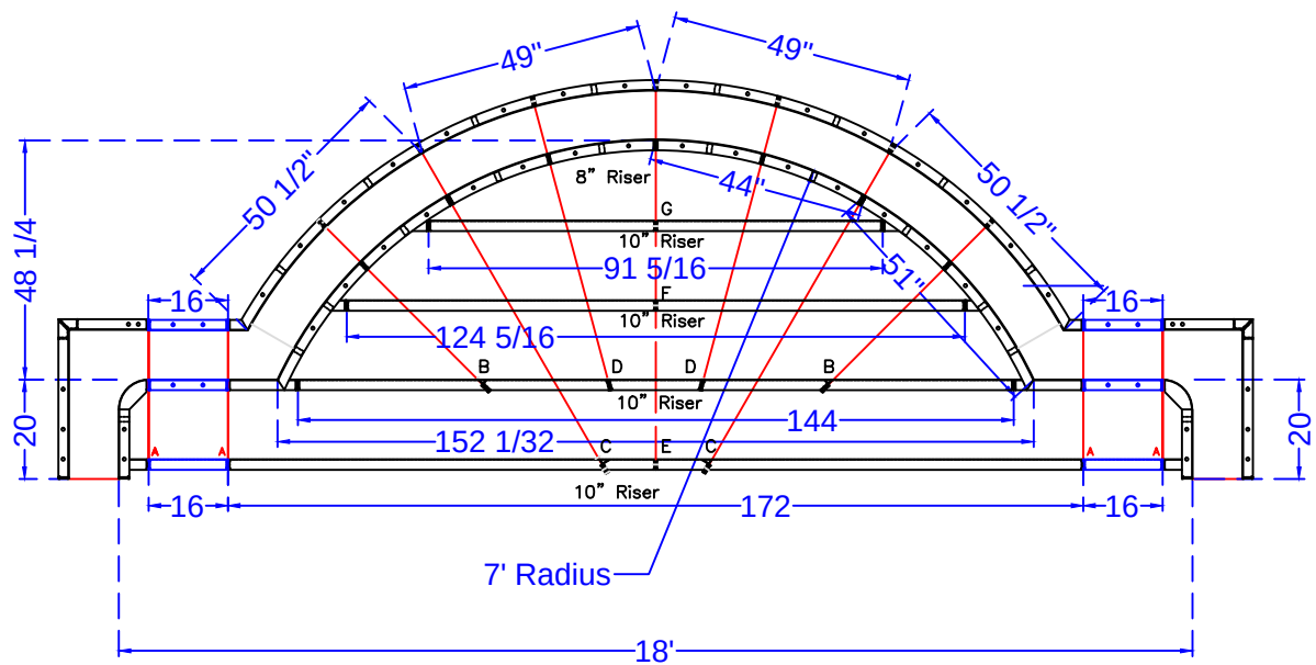
18' ROMAN END STEP ASSEMBLY SHOWN x 48 SCALE: 1' = 1/4"
