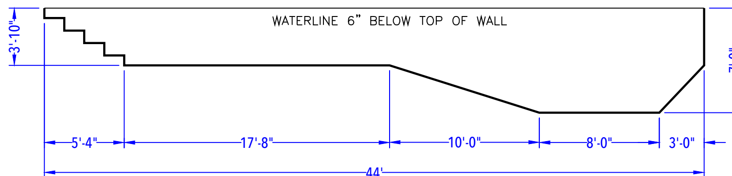
DEPTH DETAIL
