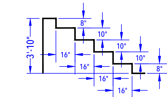
ENTRY STEP DETAIL (After Concrete & Liner) N.T.S.
