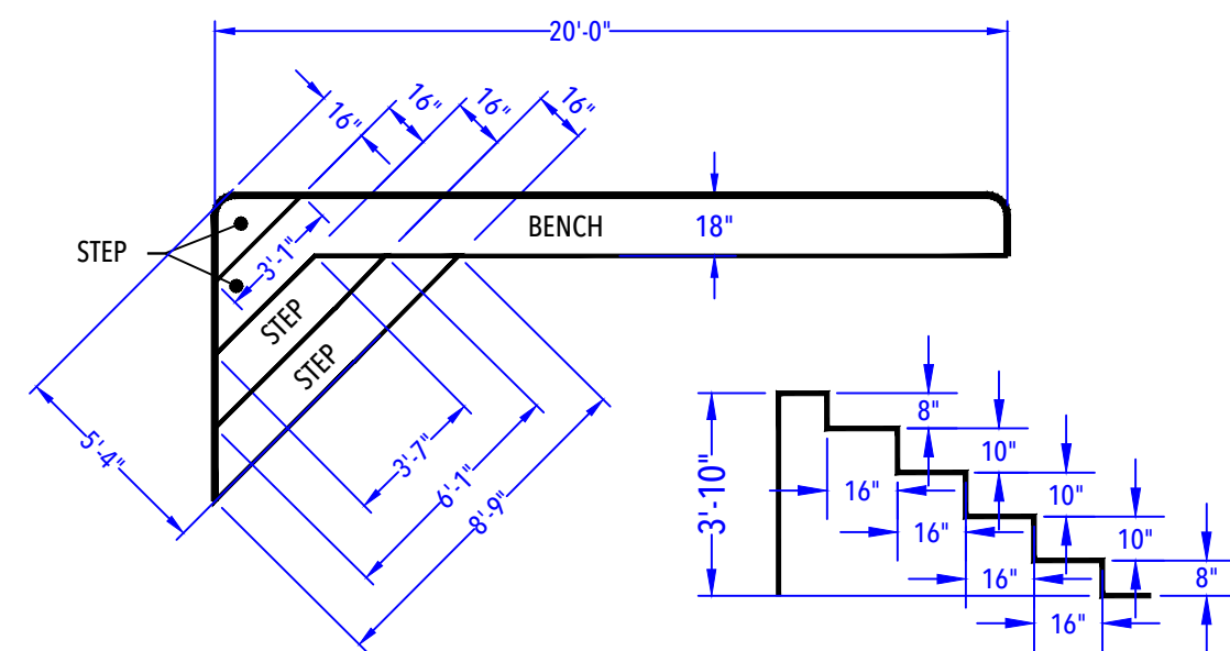
ENTRY STEP DETAIL (After Concrete & Liner) N.T.S.
