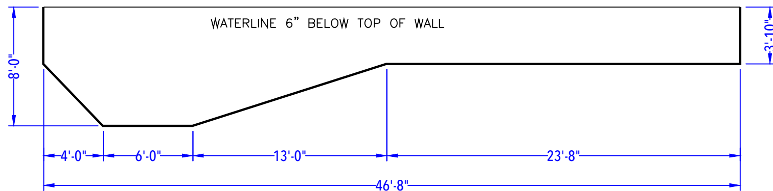
DEPTH DETAIL
