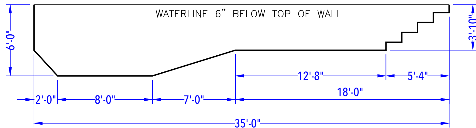
DEPTH DETAIL
