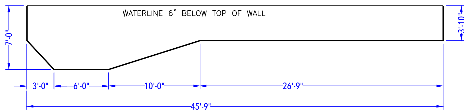
DEPTH DETAIL
