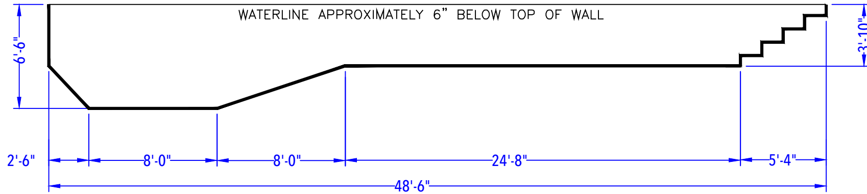
DEPTH DETAIL
